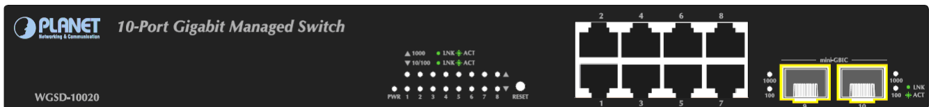
Figure 2-1 WGSD-10020 front panel.
