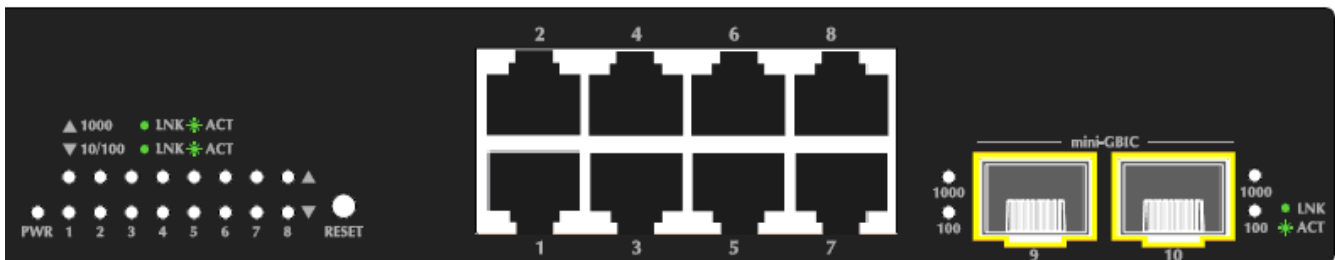
Figure 2-3 WGSD-10020 LED panel
