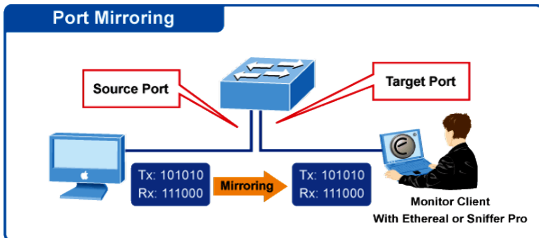
Figure 4-4-7: Port Mirror Application
