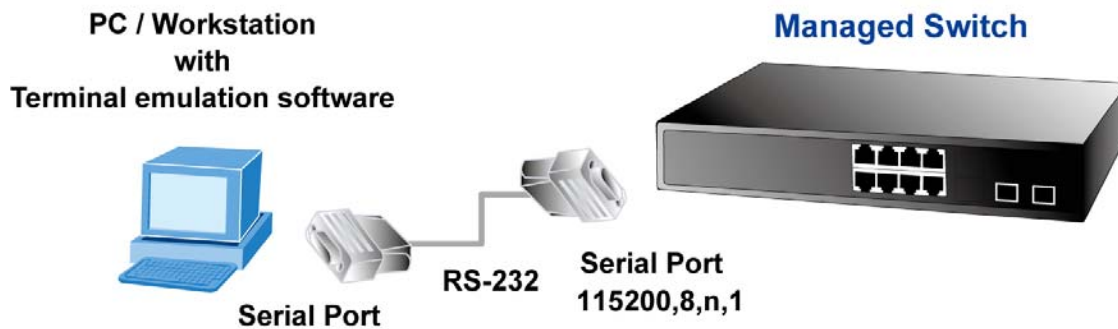
Figure 3-1-1: Console Management
