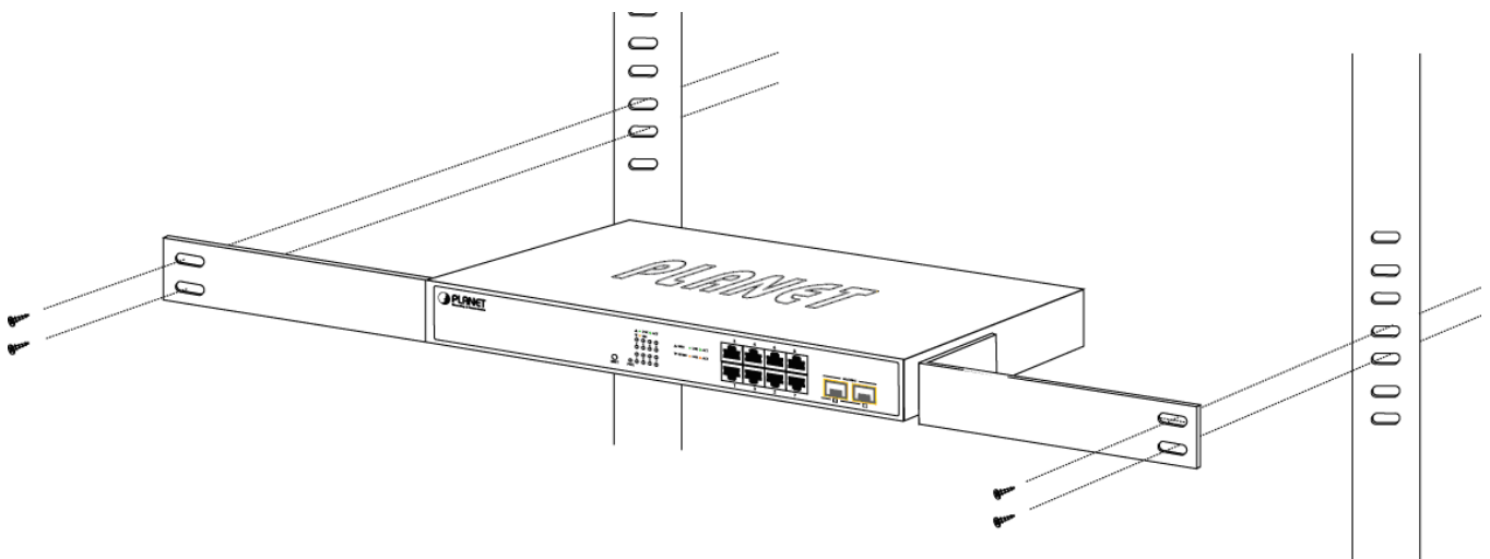
Figure 2-9 Mounting WGSD-10020 in a Rack
