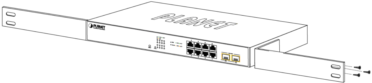
Figure 2-8 Attach brackets to the Managed Switch.
